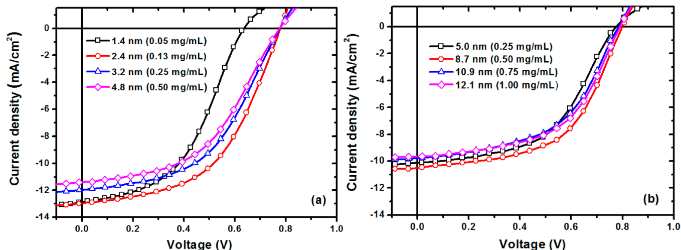
Figure 3. J – V characteristics of solar cells with various interlayer thickness under AM 1.5G irradiation at 100 \text{ mW}/\text{cm}^2 : (a) TrNBr; (b) TrOH.
